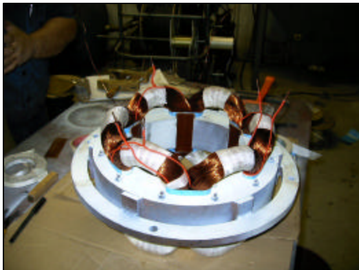
Rewind assembly ready for dip-and-bake.
